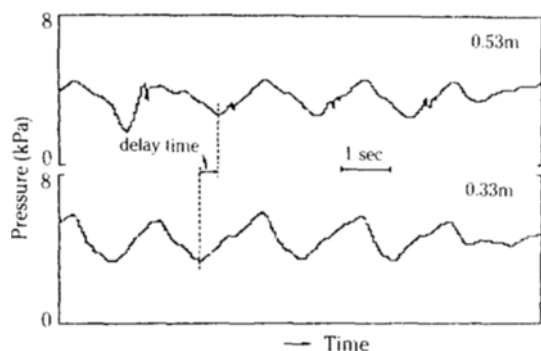
Fig. 2. Pressure fluctuation signals at a gas velocity of 0.42 m/s.
