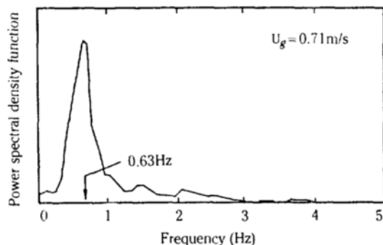
Fig. 8. Power spectral density function of pressure signals obtained at 0.53m above the distributor with a gas velocity of 0.71m/s.
