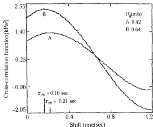
Fig. 3. Cross-correlation functions between two pressure fluctuation signals.
